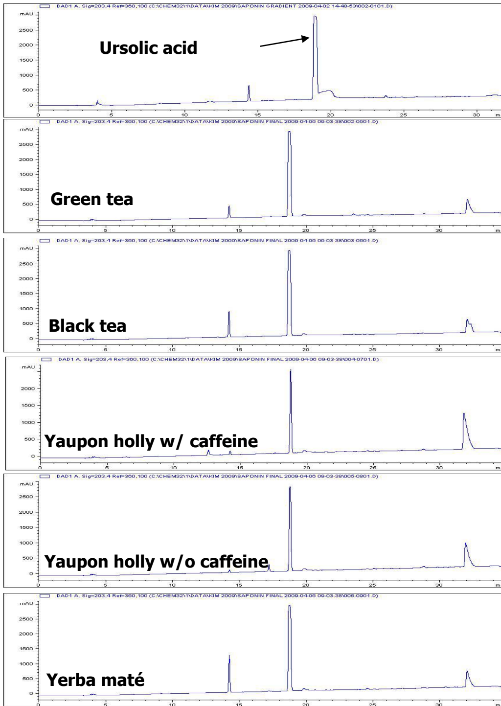
Figure 1. Chromatograms of 5 teas containing saponins. All the peaks in chromatogram represent saponin and the concentrations were expressed as Ursolic acid equivalent.
